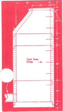
● PRE-CAST MANHOLES
